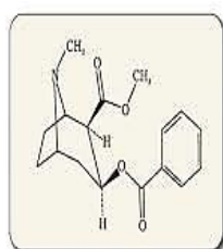
Figure 8.7 Chemical structure of Morphine
