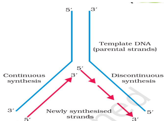
Figure 5.8 Replicating Fork
