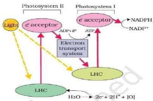
Z-scheme of Light reaction
